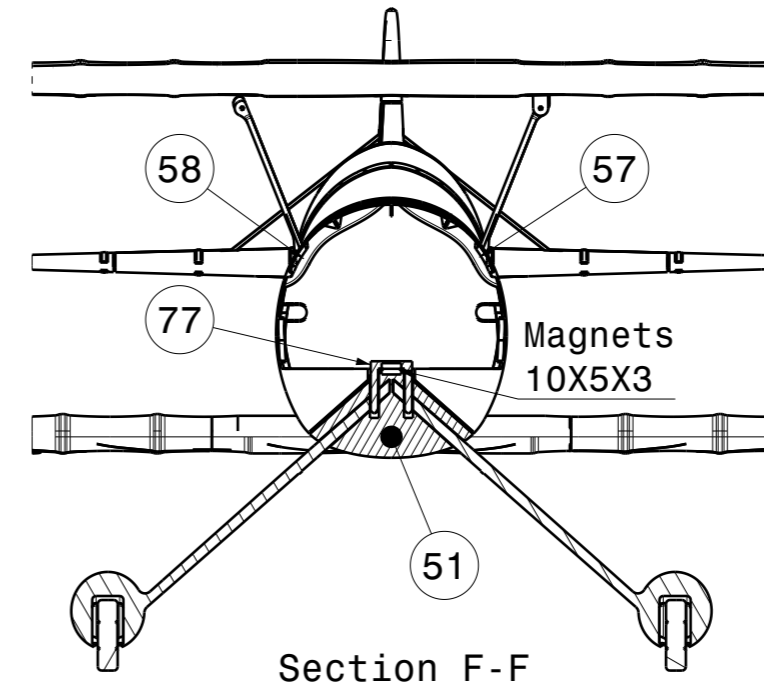
Section F-F
