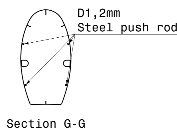
Section G-G
