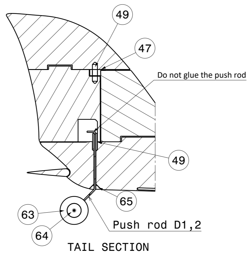
TAIL SECTION
