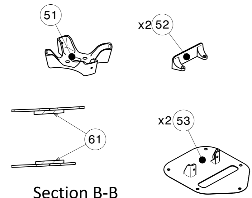
Section B-B (Concept valid also for join between WingC and Wing1R)
