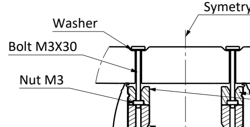
Section C-C
