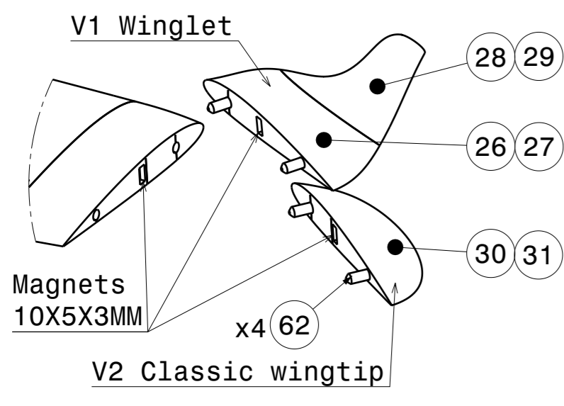
WINGTIP DETAIL
